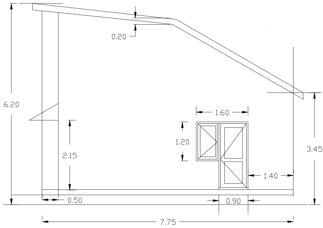
Proposed dwelling View from the East David Stonebanks MPeast4.dwg 5 May 2016 scale 1:100
